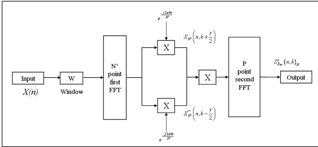
Figure 2. Block Diagram for the Cyclostationary Time-Smoothing Fast Fourier Transform Accumulation Method (From: [3]).
